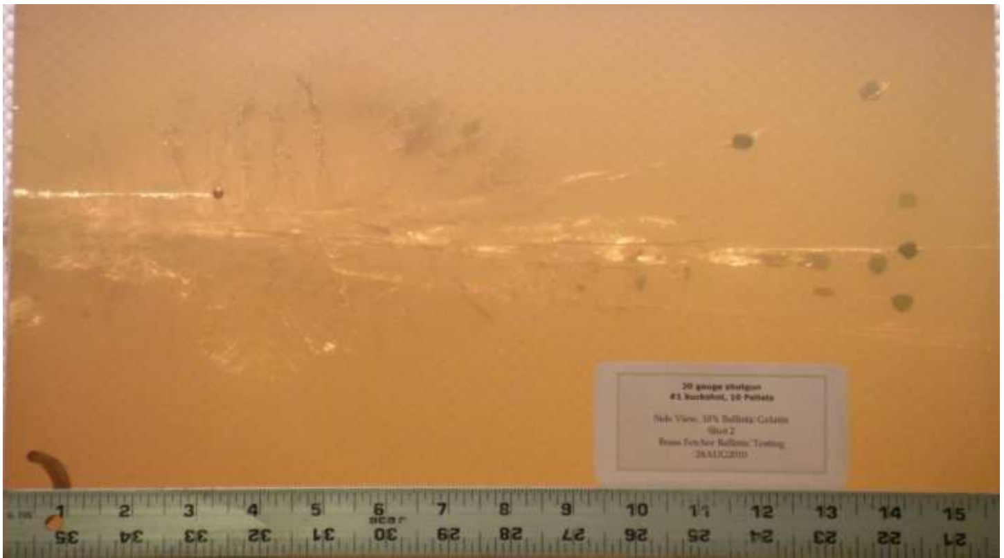
Figure 4. Side view of Shot 2 gelatin block
