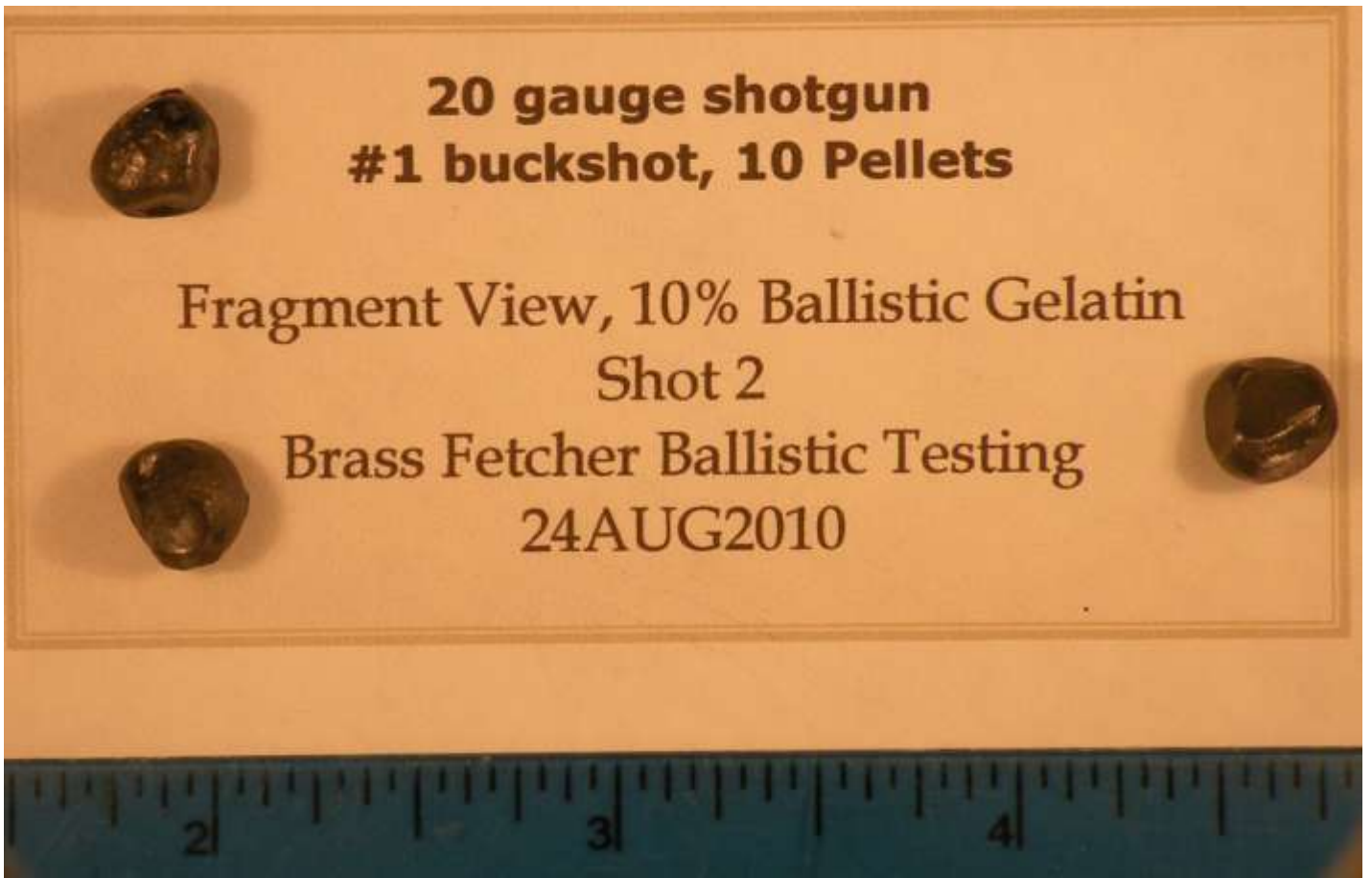
Figure 6. Fragment view of Shot 2 recovered shot pellets
