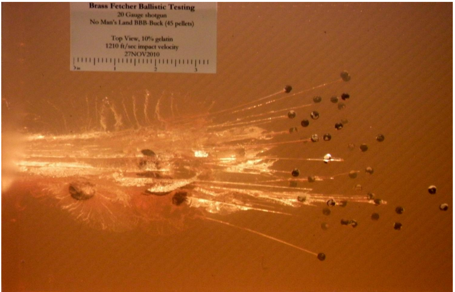
Figure 2. Top view of Shot 1 gelatin block
