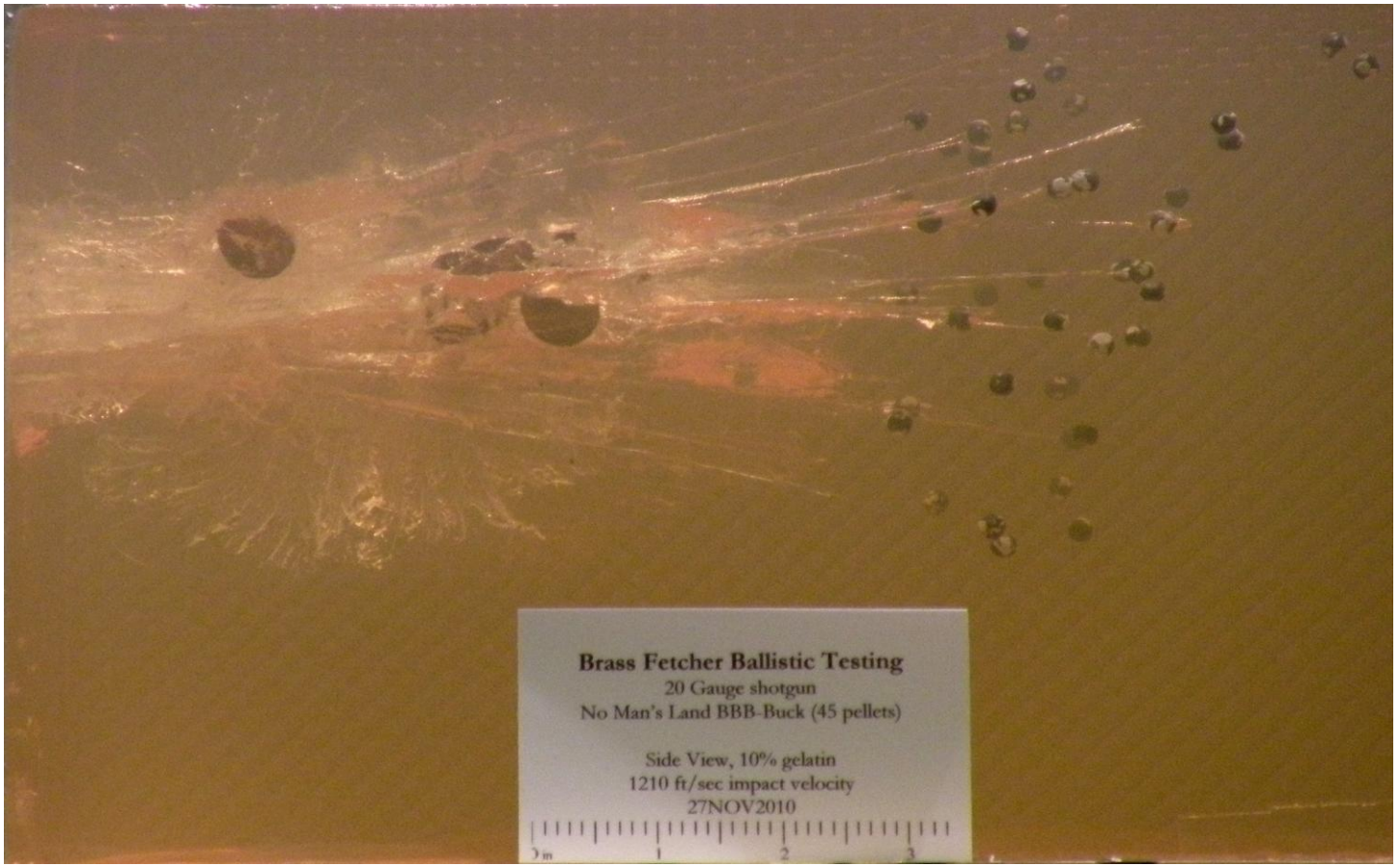
Figure 1. Side view of Shot 1 gelatin block
